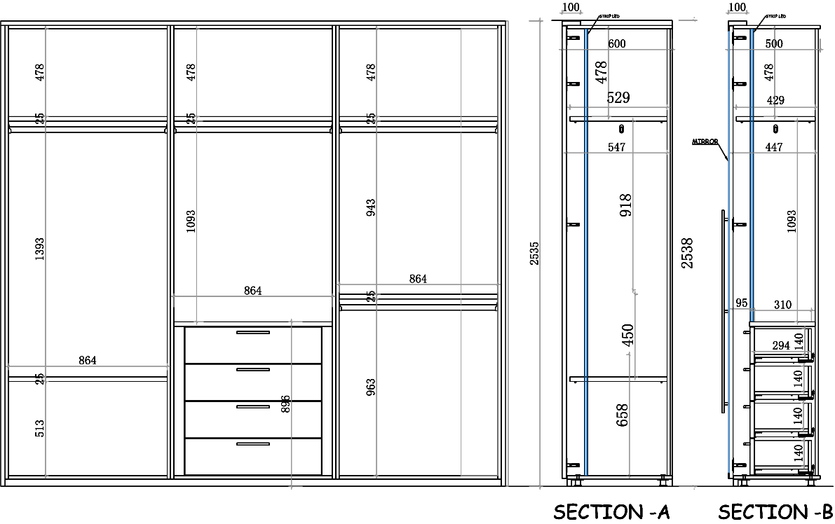
WALK IN CLOSET 3- ELEVATION 1- INNER VIEW
