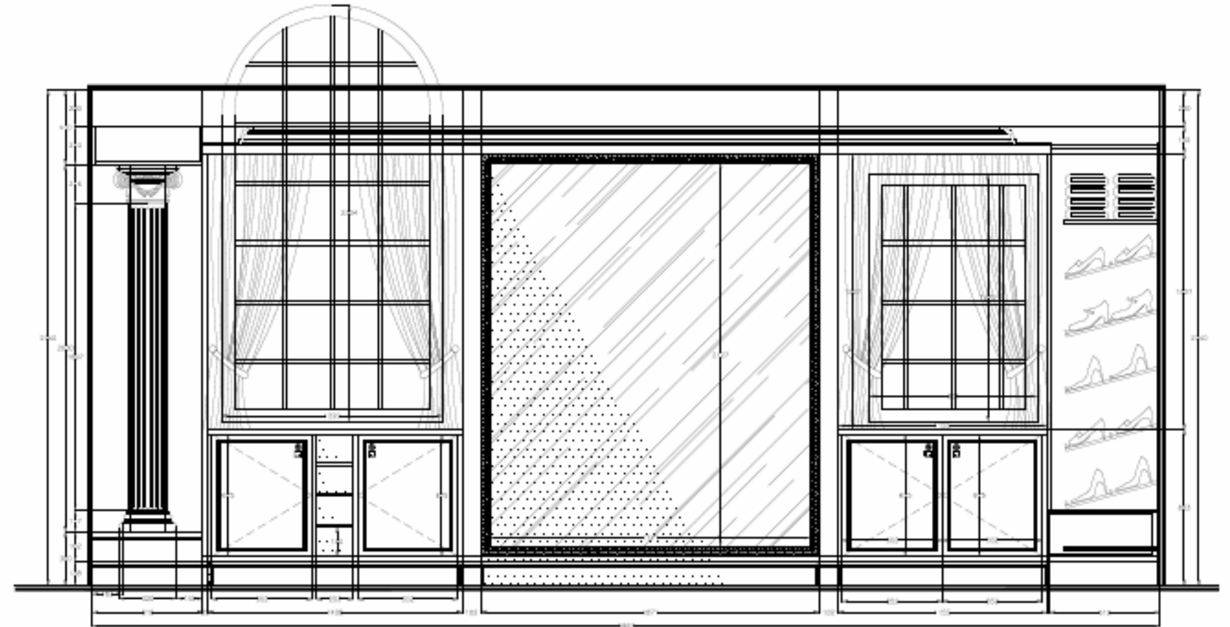
MASTER BEDROOM - WALK IN CLOSET - ELEVATION A - B
