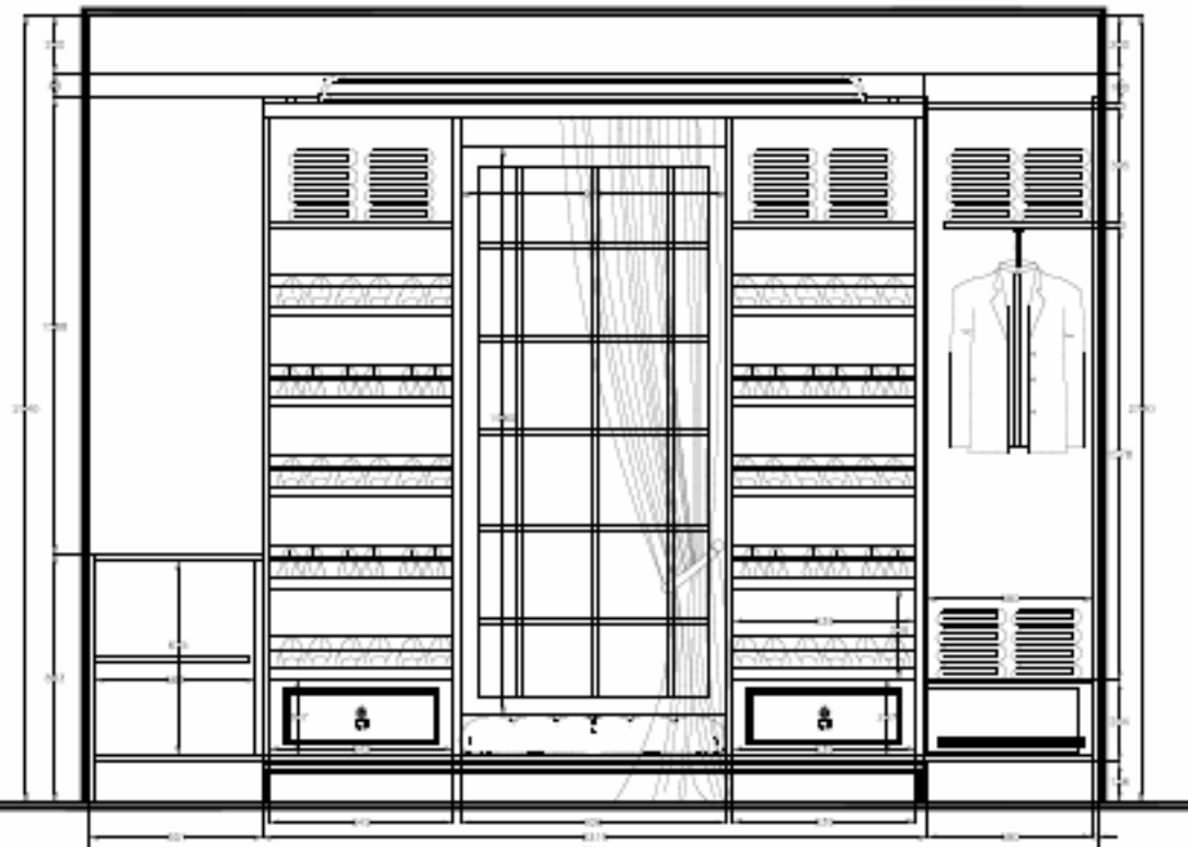
MASTER BEDROOM - WALK IN CLOSET - ELEVATION B - C
