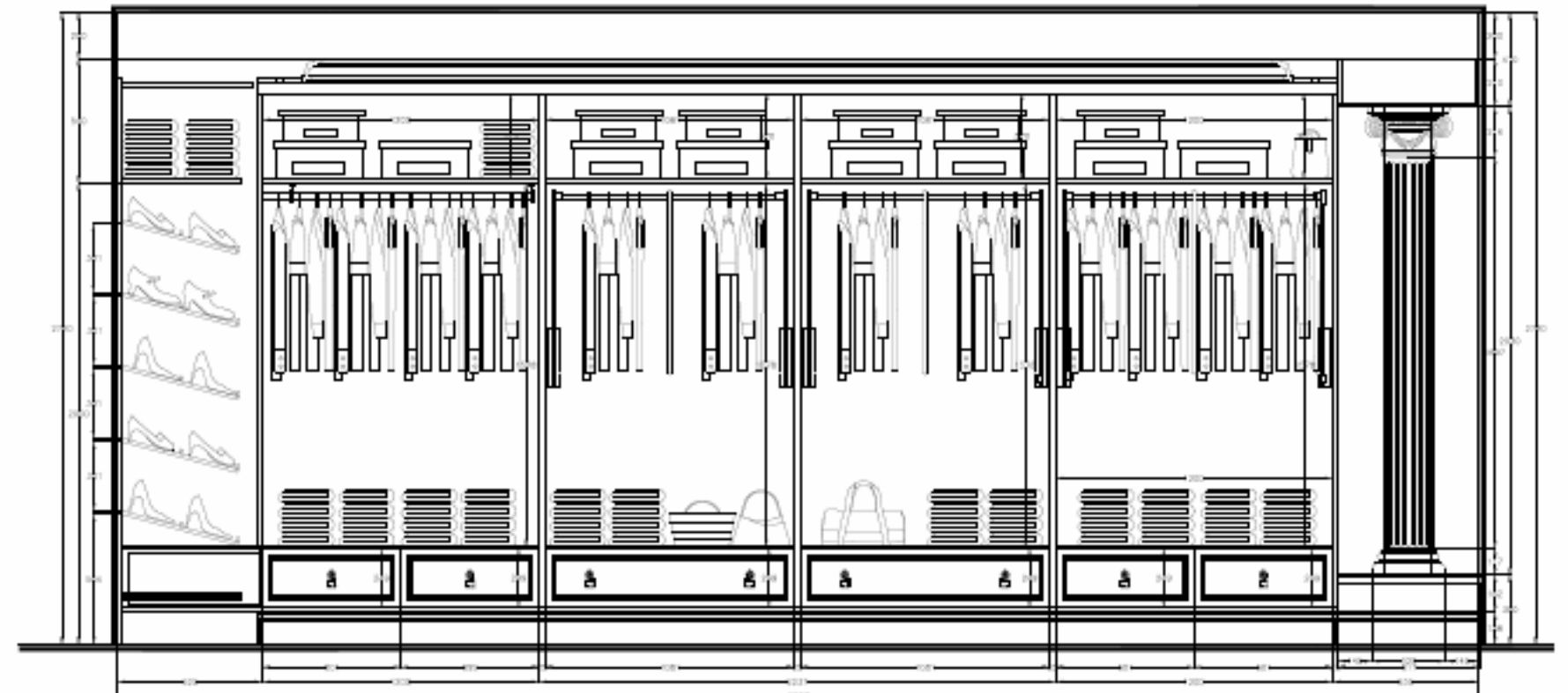
MASTER BEDROOM - WALK IN CLOSET - ELEVATION C - D
